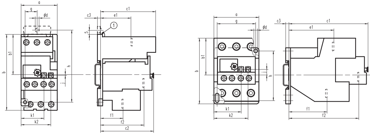
CT7N-23..37 with Panel Mount Adaptor
