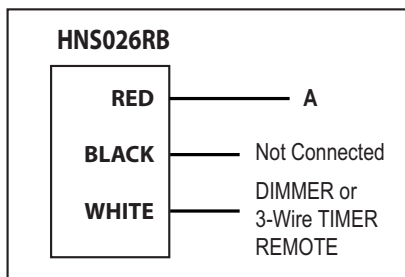
Fig 5: Button only operation
