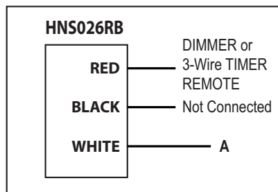
Fig 6: Button only operation
