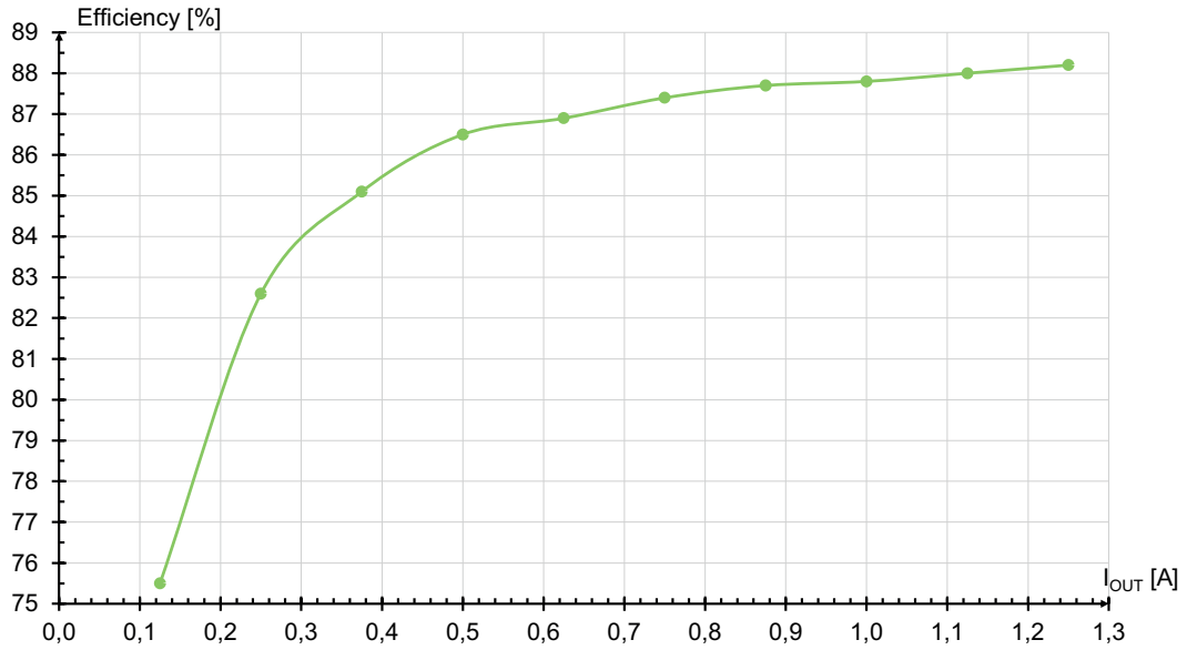
Figure 8: Efficiency at 230 VAC
