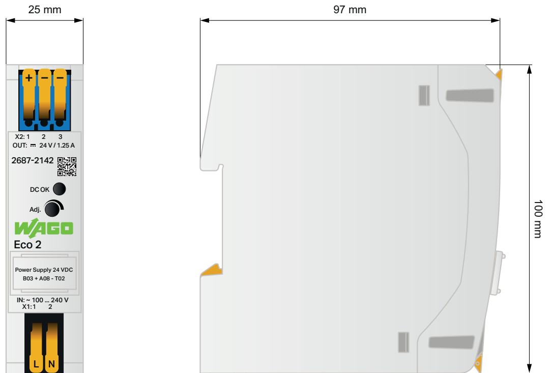
Figure 7: Dimensions
