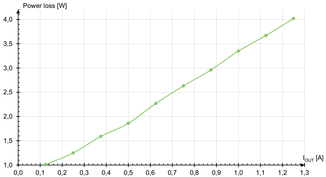
Figure 9: Power loss at 230 VAC
