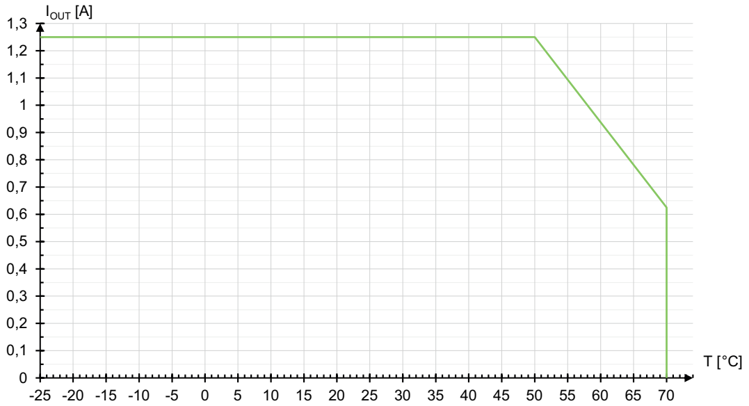
Figure 10: Derating (Temperature-Dependent)
