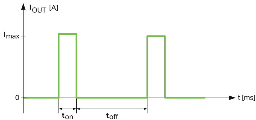
Figure 11: Hiccup-Mode
