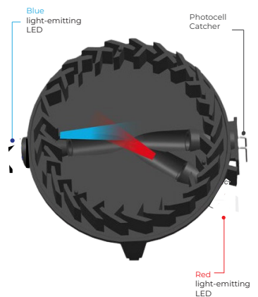
Split-spectrum smoke chamber Distinguish smoke from vapour or dust to eliminate false alarm
