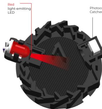
Traditional Smoke Chamber
