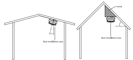
Figure 4 -3 Installation position (2)
