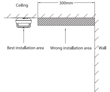
Figure 4 -2 Installation position (1)
