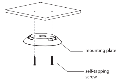
Figure 4 -4 Installation step (1)
