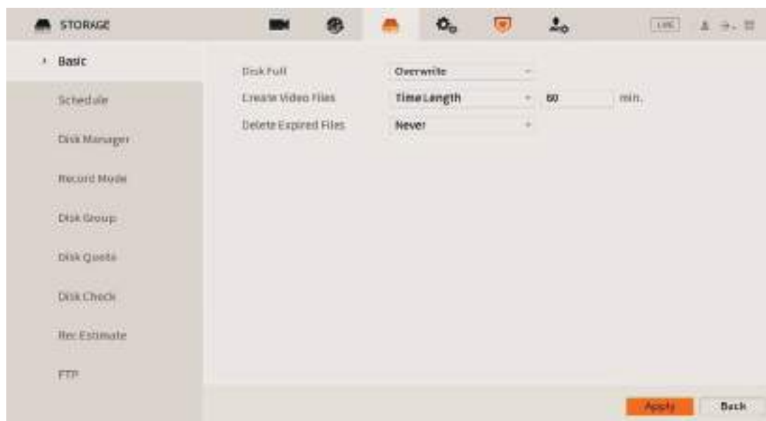
Fig. 3.13: Storage Settings
